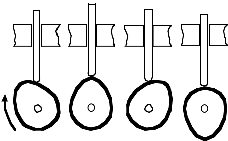
The cam follower is rising The cam follower is at its highest point The cam follower is descending The cam follower is stationary as it follows the circumference or dwell angle
