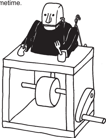
This automata is called the "Angry Diner". He rapidly bangs his knife and fork on the table, impatient for his dinner. His arms act as levers, amplifying the lift from the cam.
